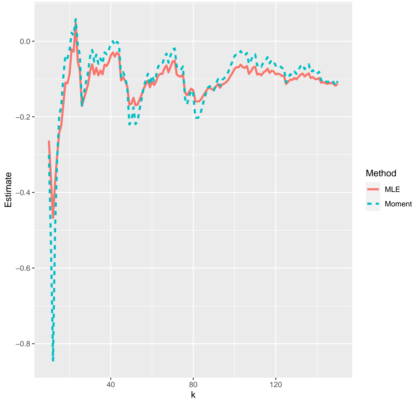
Estimates of extreme value index--04-01-2022
