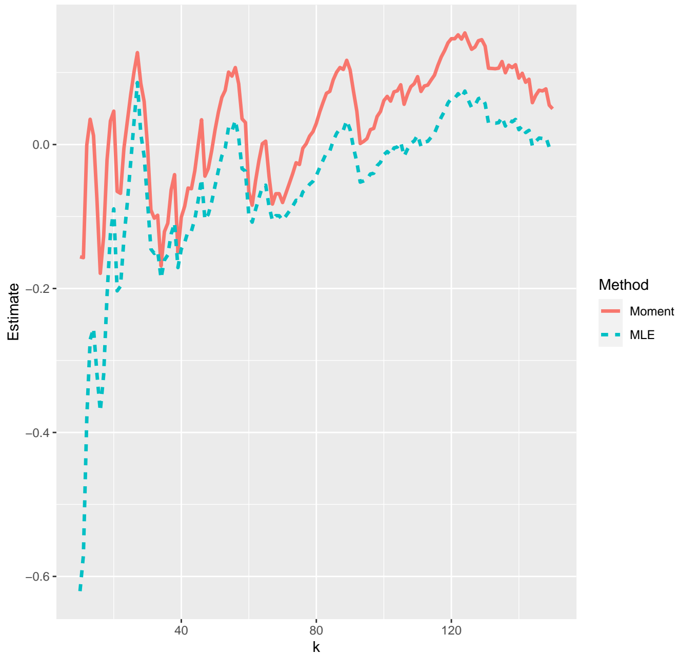
Estimates of extreme value index--03-05-2020
