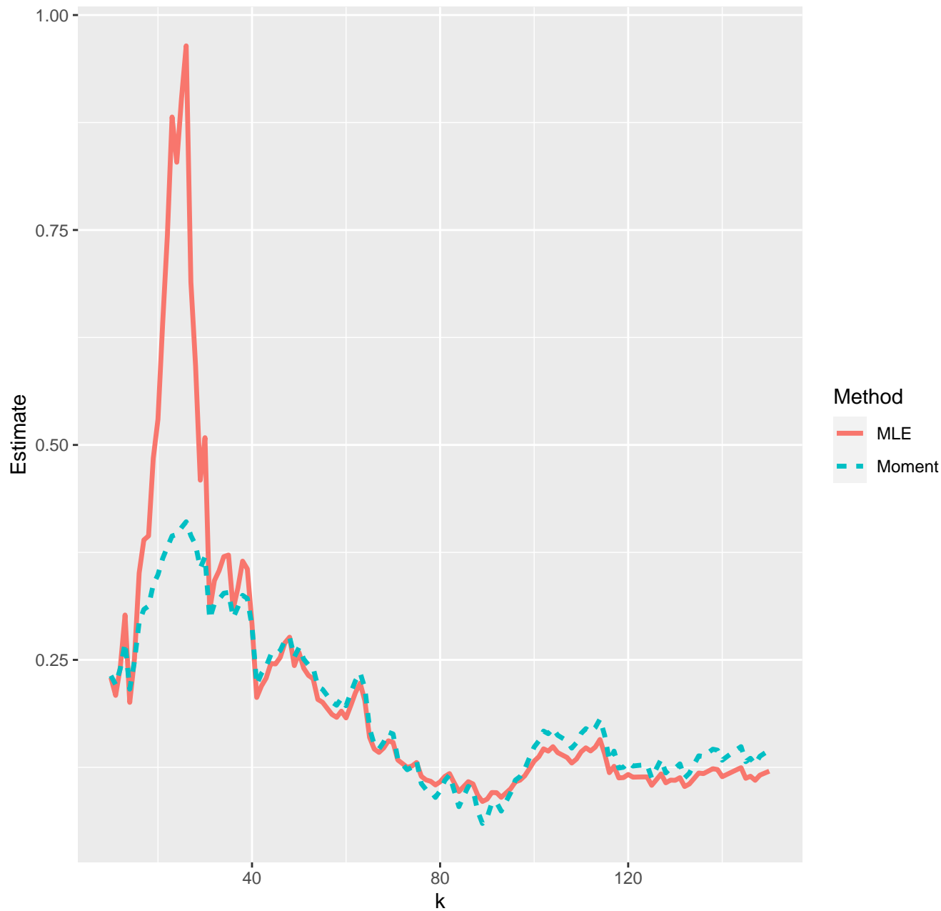
Estimates of extreme value index--03-01-2023
