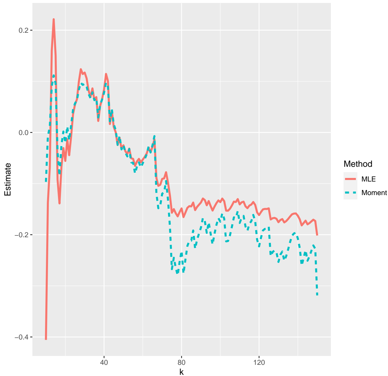
Estimates of extreme value index--02-02-2022
