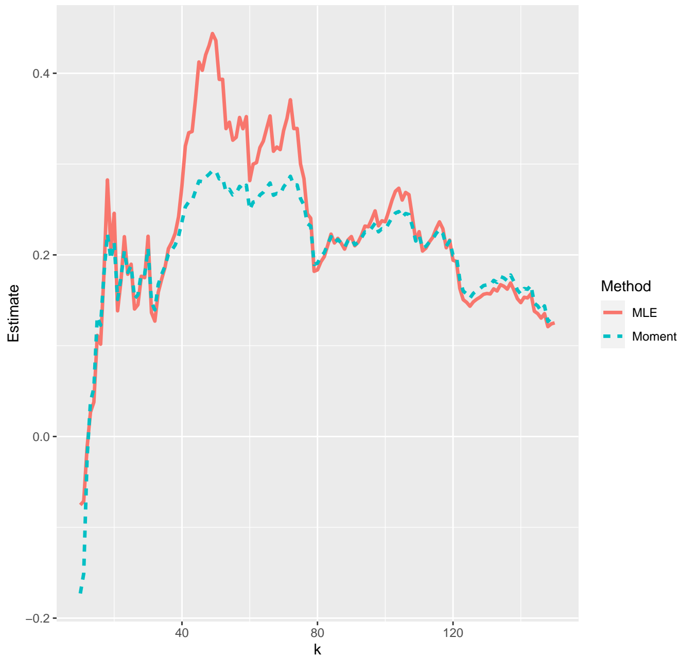
Estimates of extreme value index--01-03-2022
