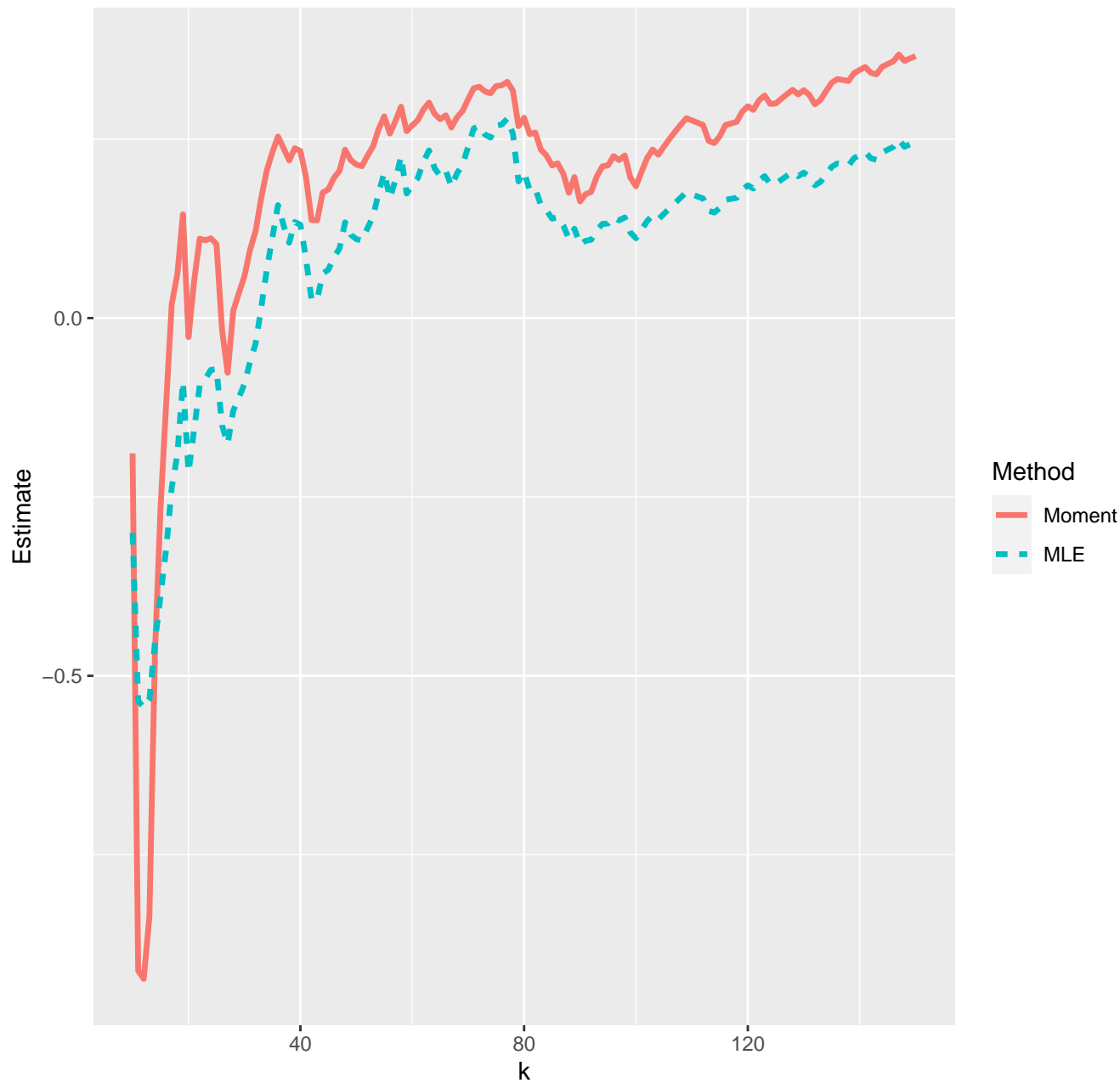
Estimates of extreme value index--31-03-2020
