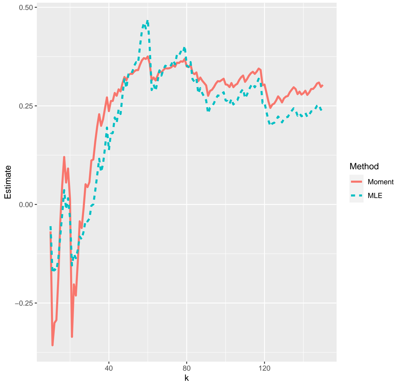
Estimates of extreme value index--30-03-2020
