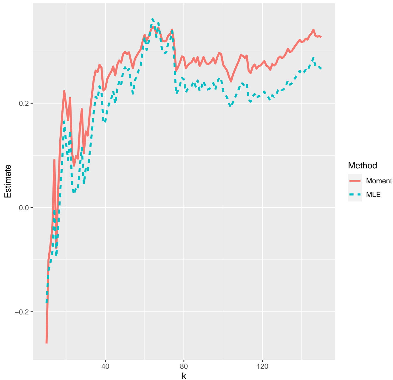
Estimates of extreme value index--28-03-2020
