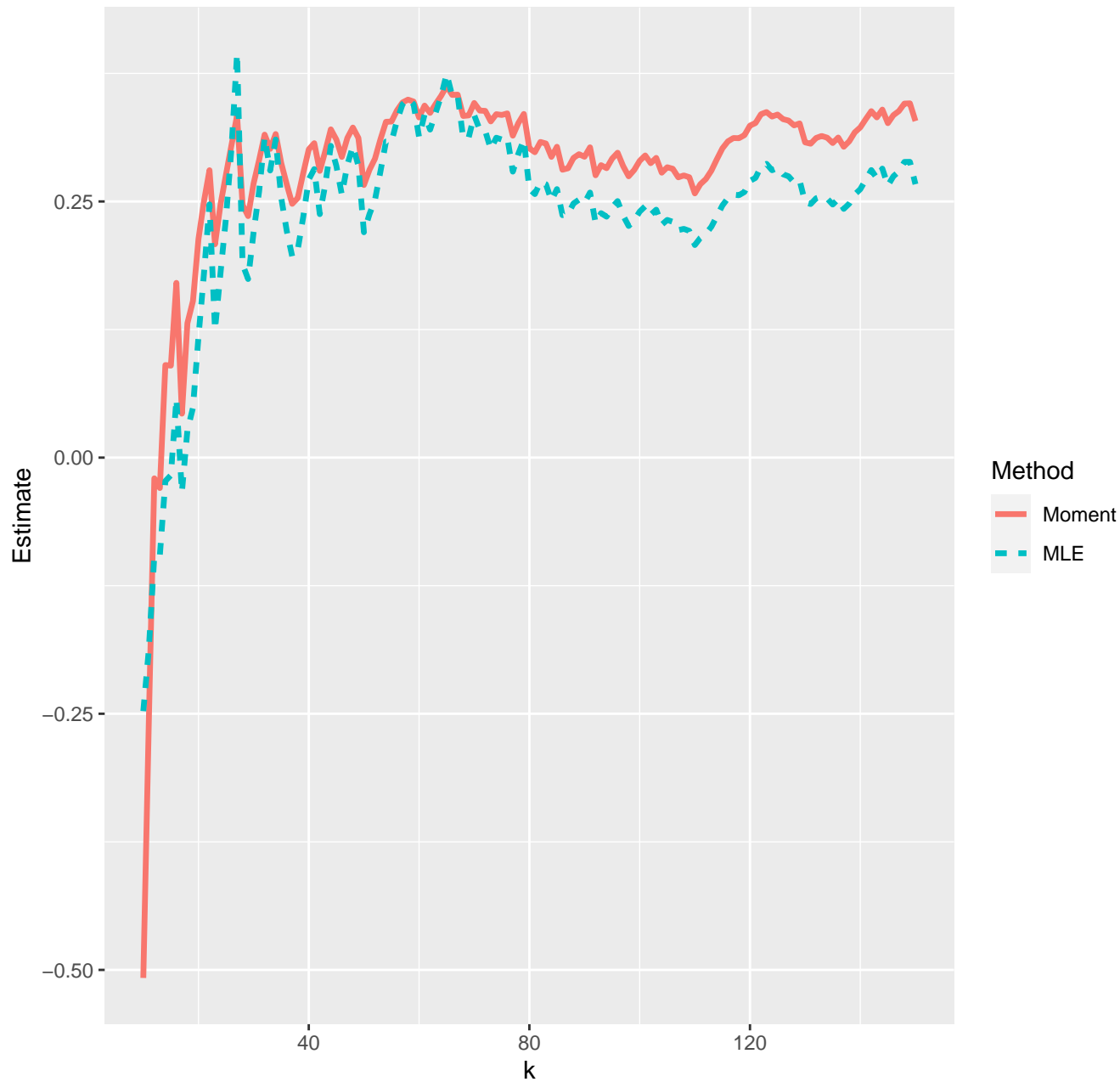
Estimates of extreme value index--27-03-2020
