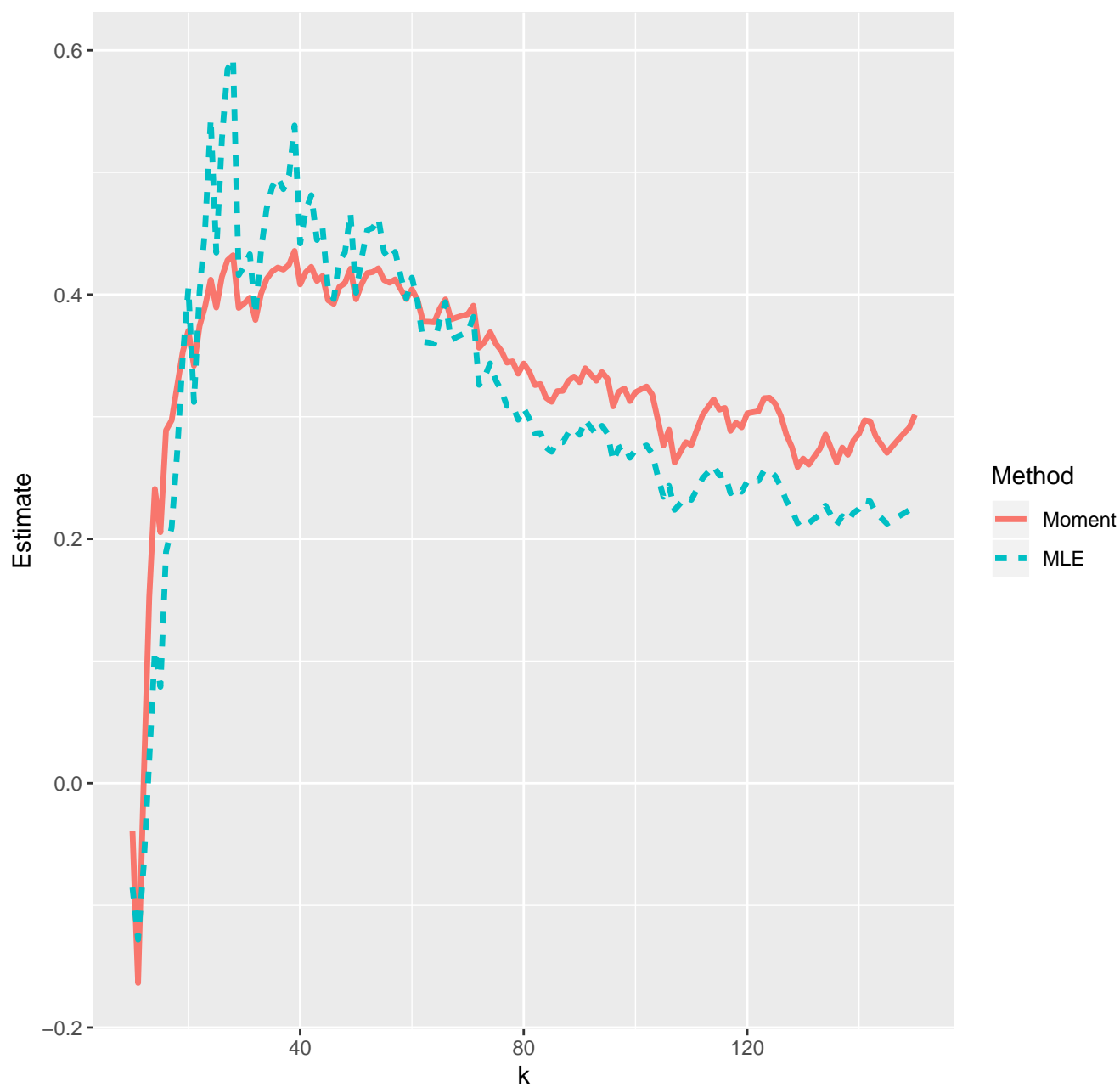
Estimates of extreme value index--24-03-2020
