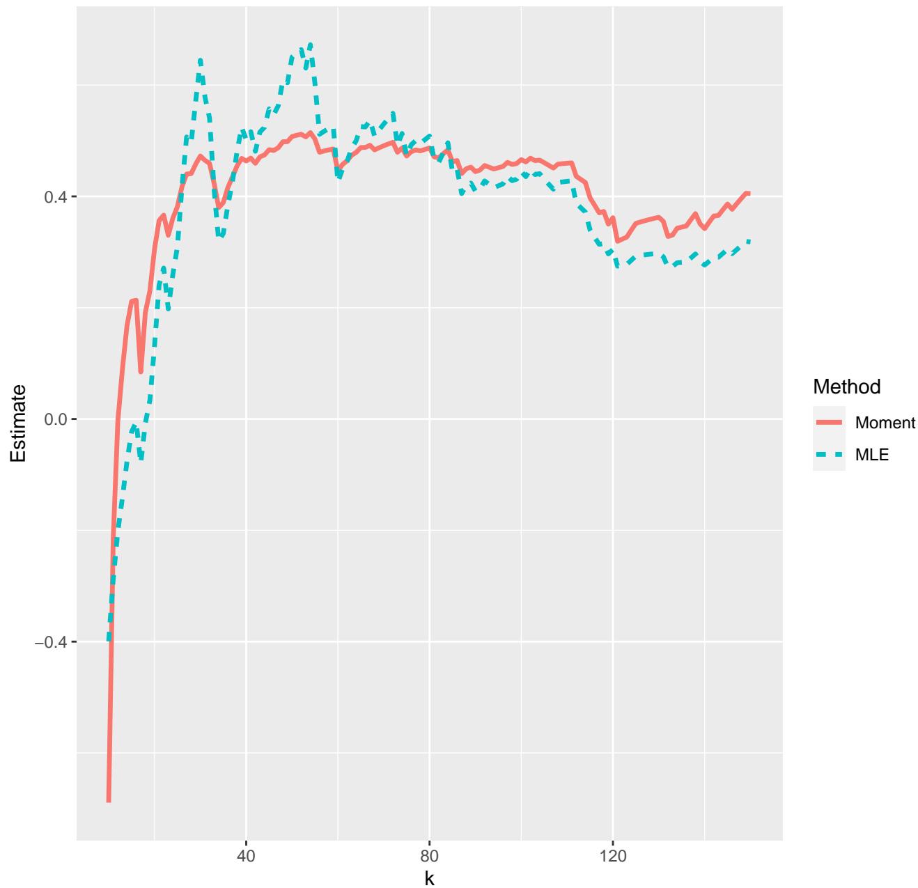
Estimates of extreme value index--20-03-2020
