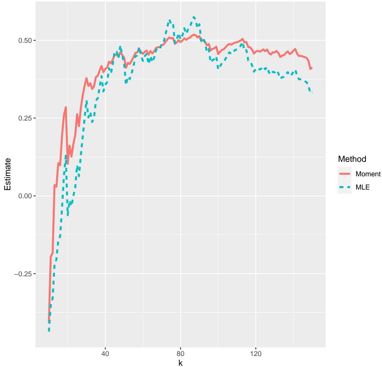
Estimates of extreme value index--19-03-2020
