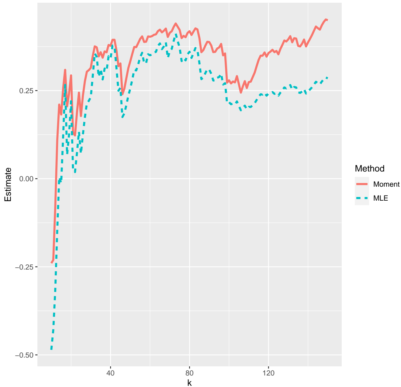
Estimates of extreme value index--17-03-2020
