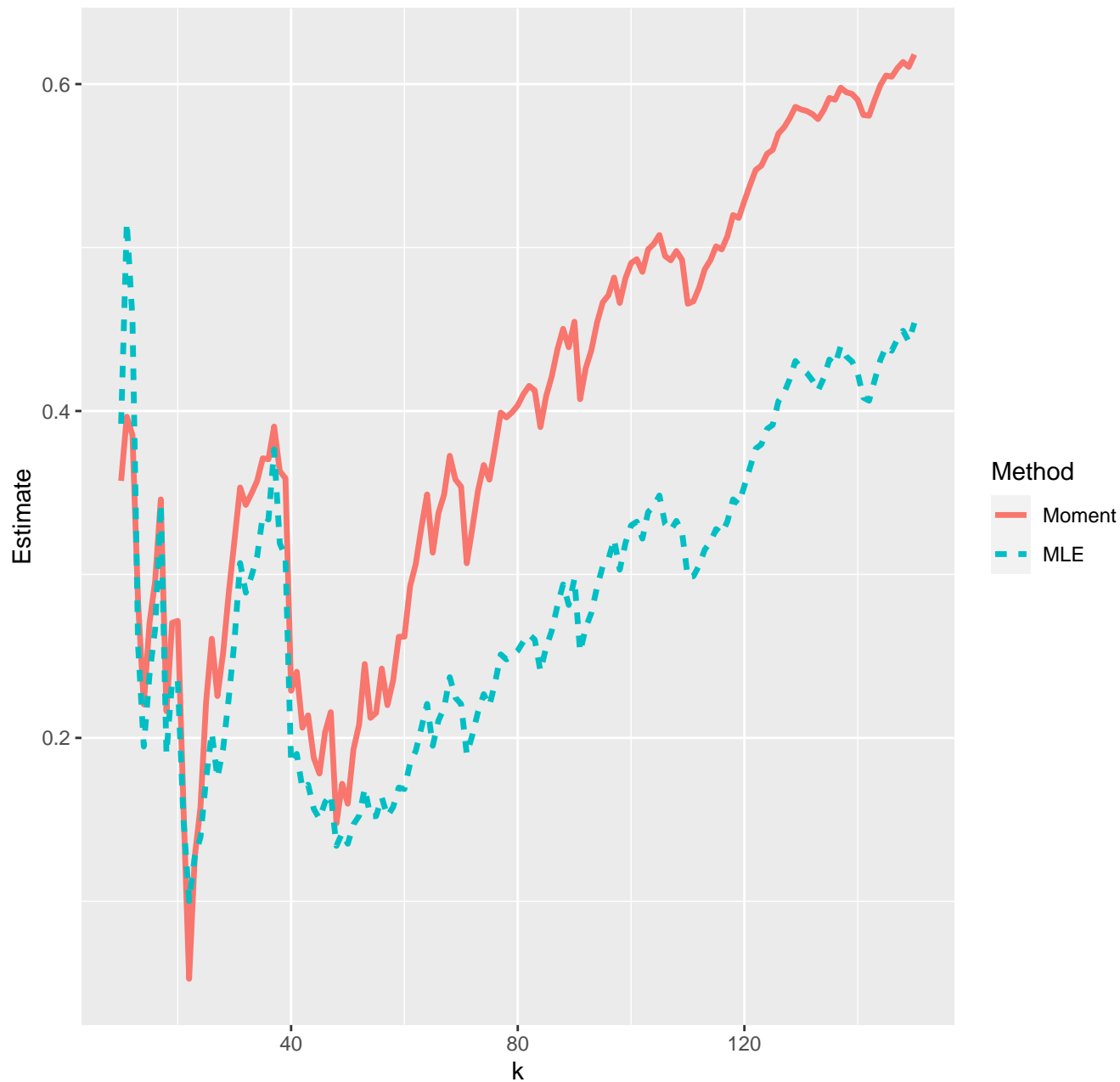
Estimates of extreme value index--14-03-2020
