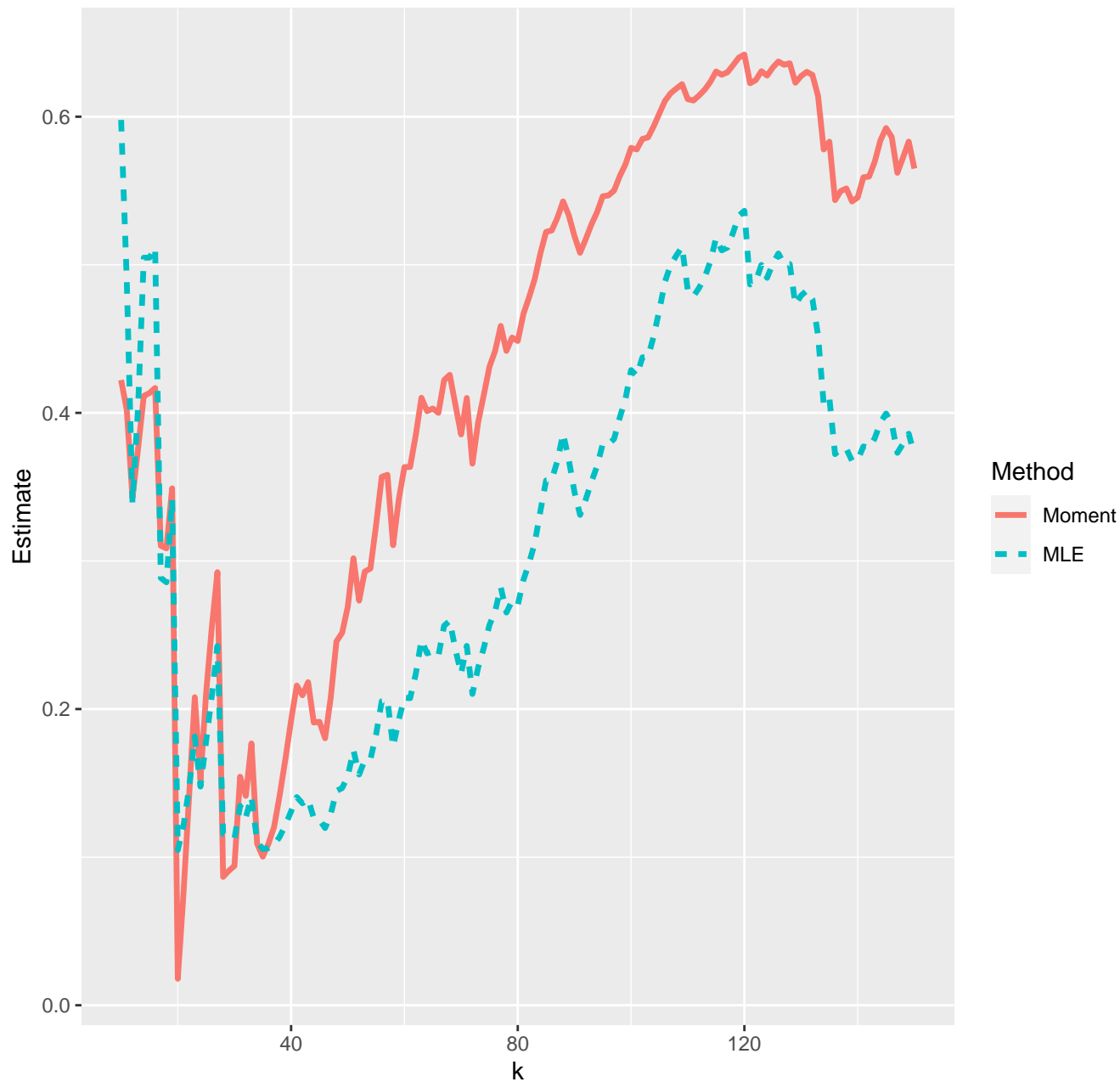
Estimates of extreme value index--13-03-2020
