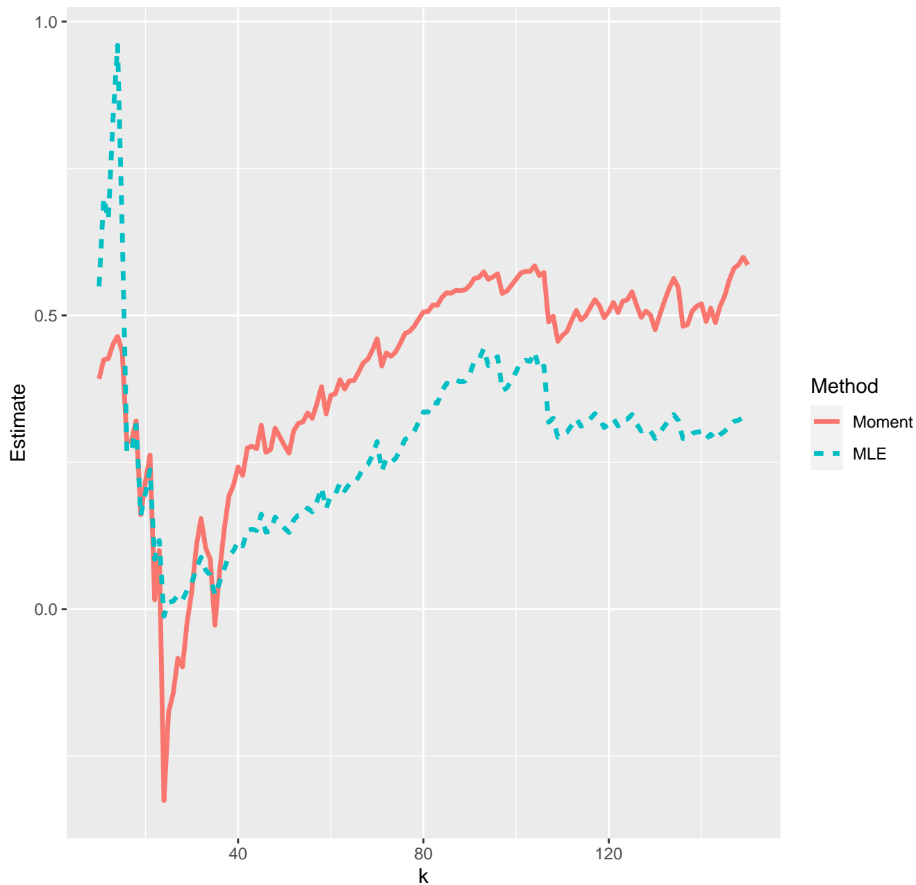
Estimates of extreme value index--12-03-2020
