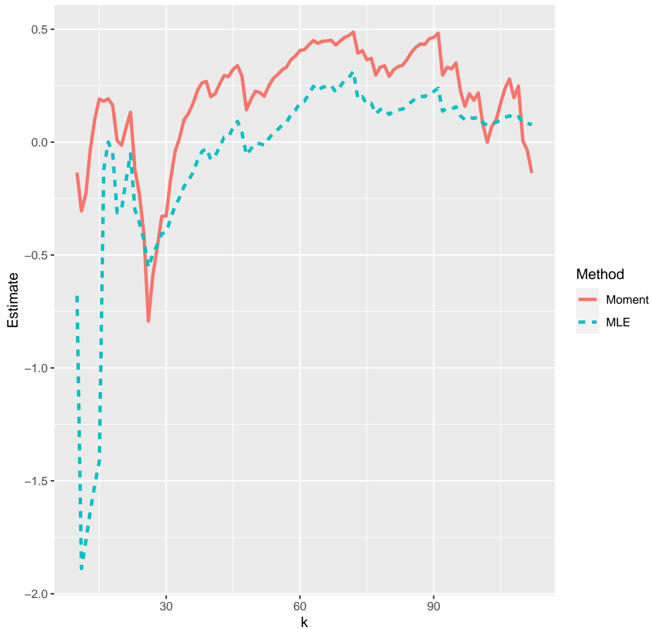
Estimates of extreme value index--10-03-2020
