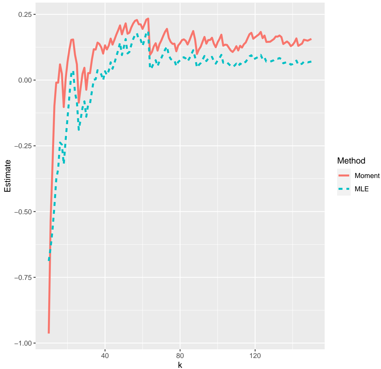
Estimates of extreme value index--07-04-2020
