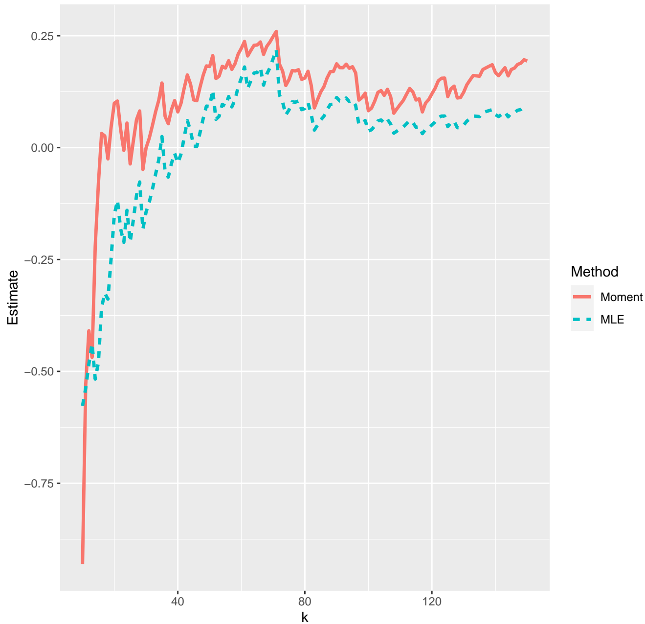
Estimates of extreme value index--06-04-2020
