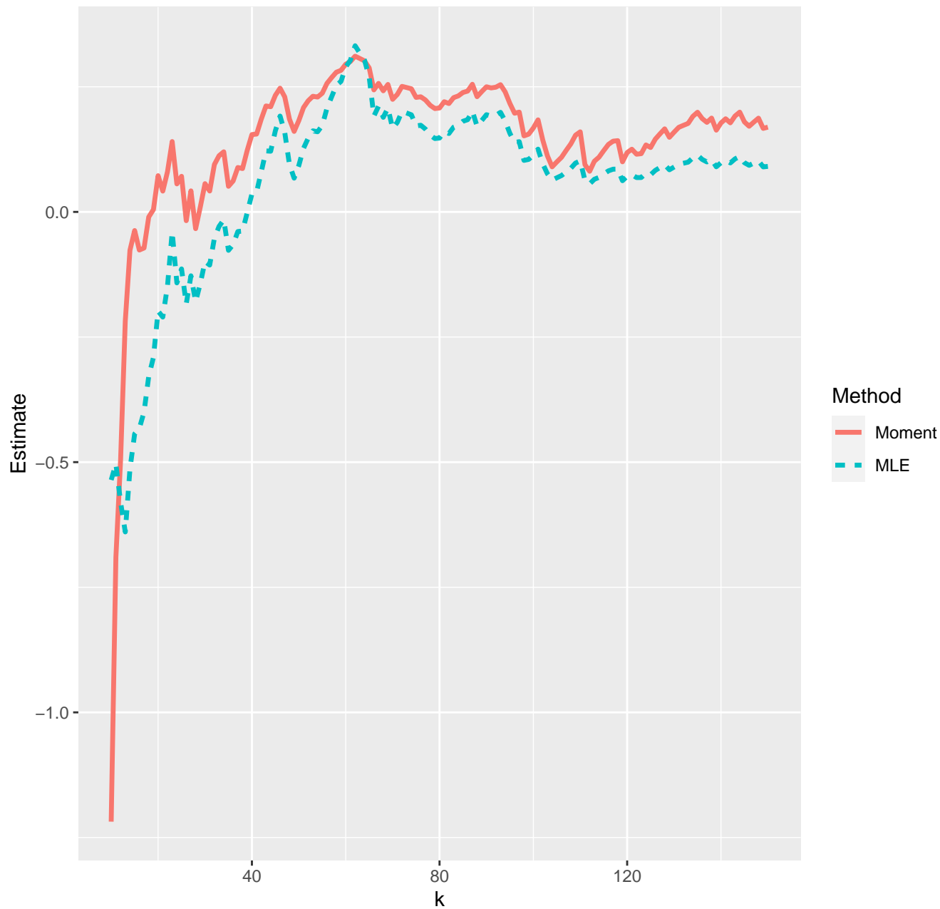
Estimates of extreme value index--05-04-2020
