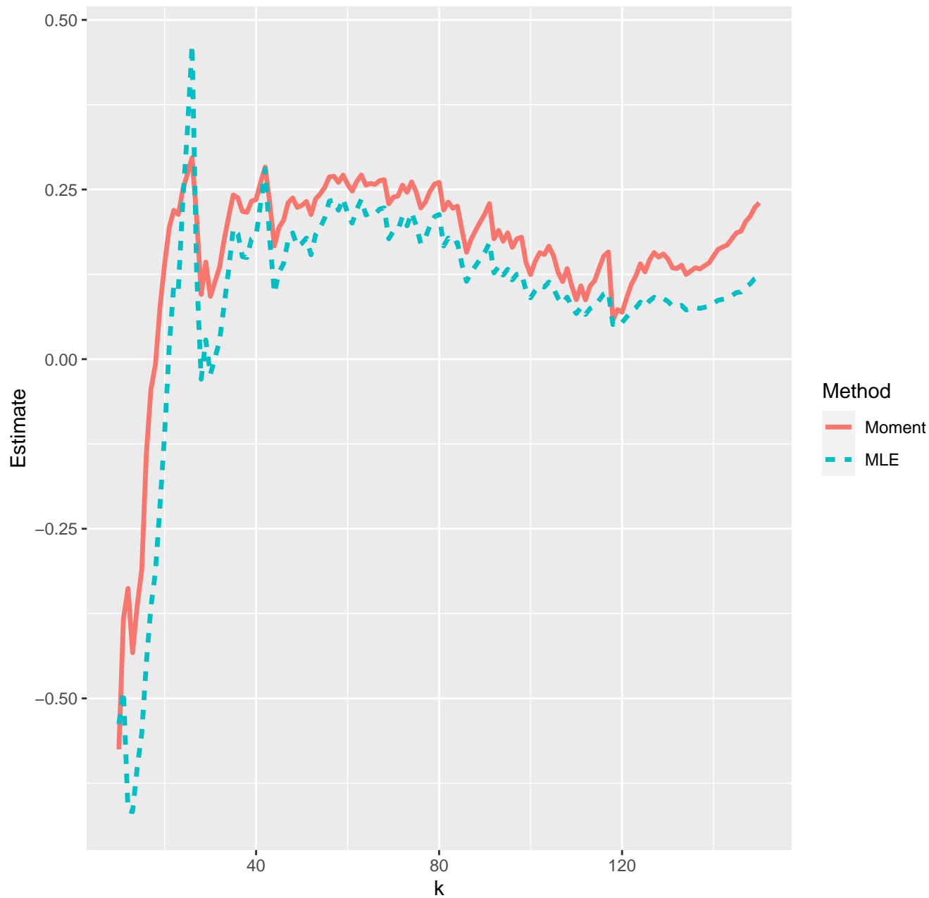
Estimates of extreme value index--03-04-2020
