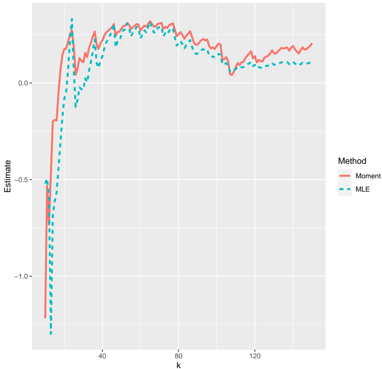
Estimates of extreme value index--02-04-2020
